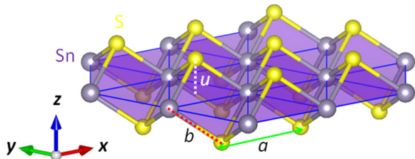
FIG. 1. Atomic structure of ML-SnS 2 . The single layer is built up from two trigonal pyramids. The structural parameters are defined in the text.
