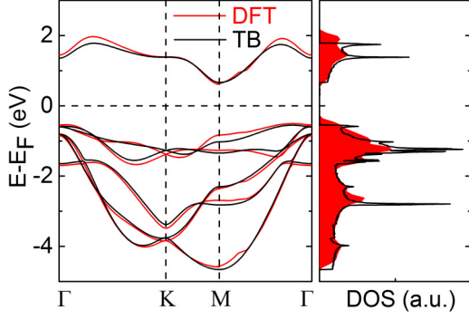
FIG. 4. Band structure (left) and density of states (right) calculated for ML-SnS 2 using the DFT and simple TB model presented in this work.
