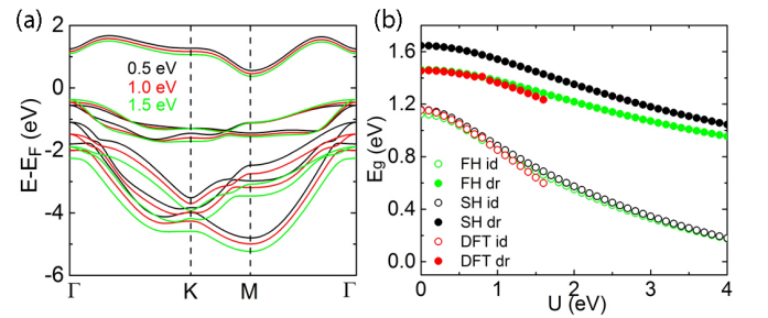
FIG. 5. Tunable electronic properties of ML-SnS 2 with external gate voltage. (a) Band structures of ML-SnS 2 calculated for different magnitudes of the gate voltage. (b) Band-gap modulation of ML-SnS 2 . The red, black, and green symbols represent the DFT, simple Hamiltonian, and full Hamiltonian results, respectively. The solid and hollow symbols indicate the direct and indirect band gap, respectively.
