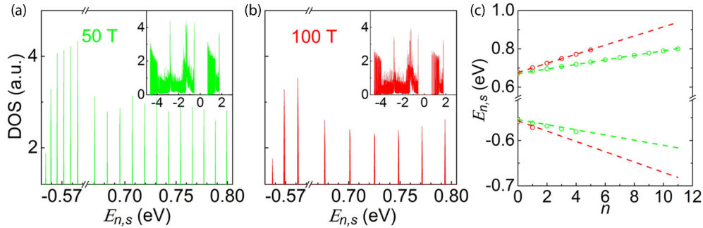
FIG. 6. Discrete Landau levels in ML-SnS 2 . A super cell of ML-SnS 2 containing 4.344 million atoms ( 3 \times 1200 \times 1200 ) is simulated in the presence of a perpendicular magnetic field. The obtained DOS in the low-energy region with magnetic fields B = 50 and 100 T are indicated by green (a) and red (b) lines. The inset shows the density of states in a wider energy window. (c) Original (circles) and numerical fitting (dashed lines) of Landau levels in ML-SnS 2 .
