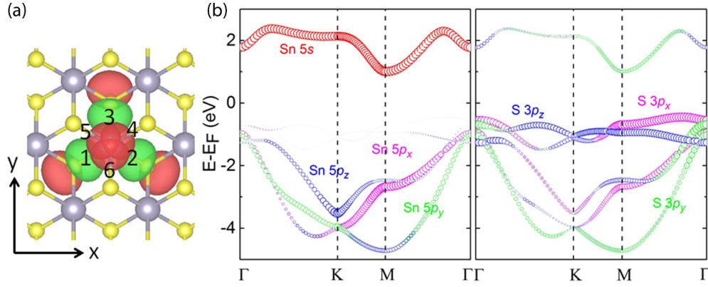
FIG. 2. Orbital characters of ML-SnS 2 . (a) Wannier orbitals of ML-SnS 2 corresponding to the basis of the TB Hamiltonian presented in this work. For clarity, orbitals are shown for one S-atom sublattice with three orbitals per atom. The orbitals in the second sublattice are symmetric with respect to the inversion center. (b) Orbital decomposed band structure of Sn and S in ML-SnS 2 , with the corresponding s , p x , p y , and p z orbitals being red, pink, green, and blue, respectively. The size of the symbol represents the orbital weight.
