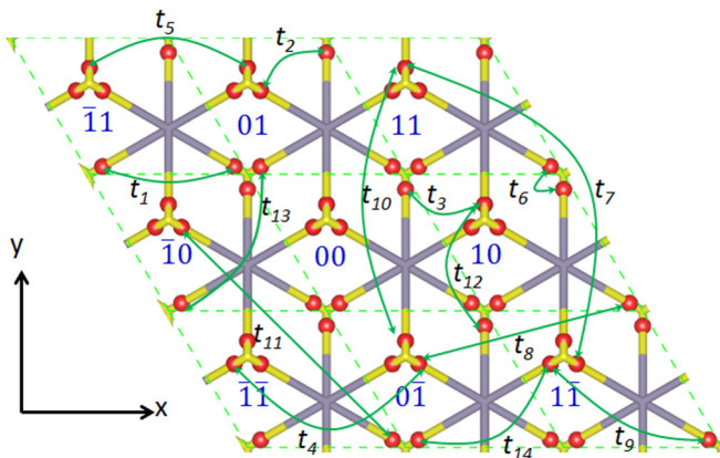
FIG. 3. Schematic diagram of the relevant hopping parameters ( t_i ) involved in our simple TB model of ML-SnS 2 . Interacting hopping centers are indicated by red balls, corresponding to the negative part of the Wannier orbitals shown in Fig. 2.
